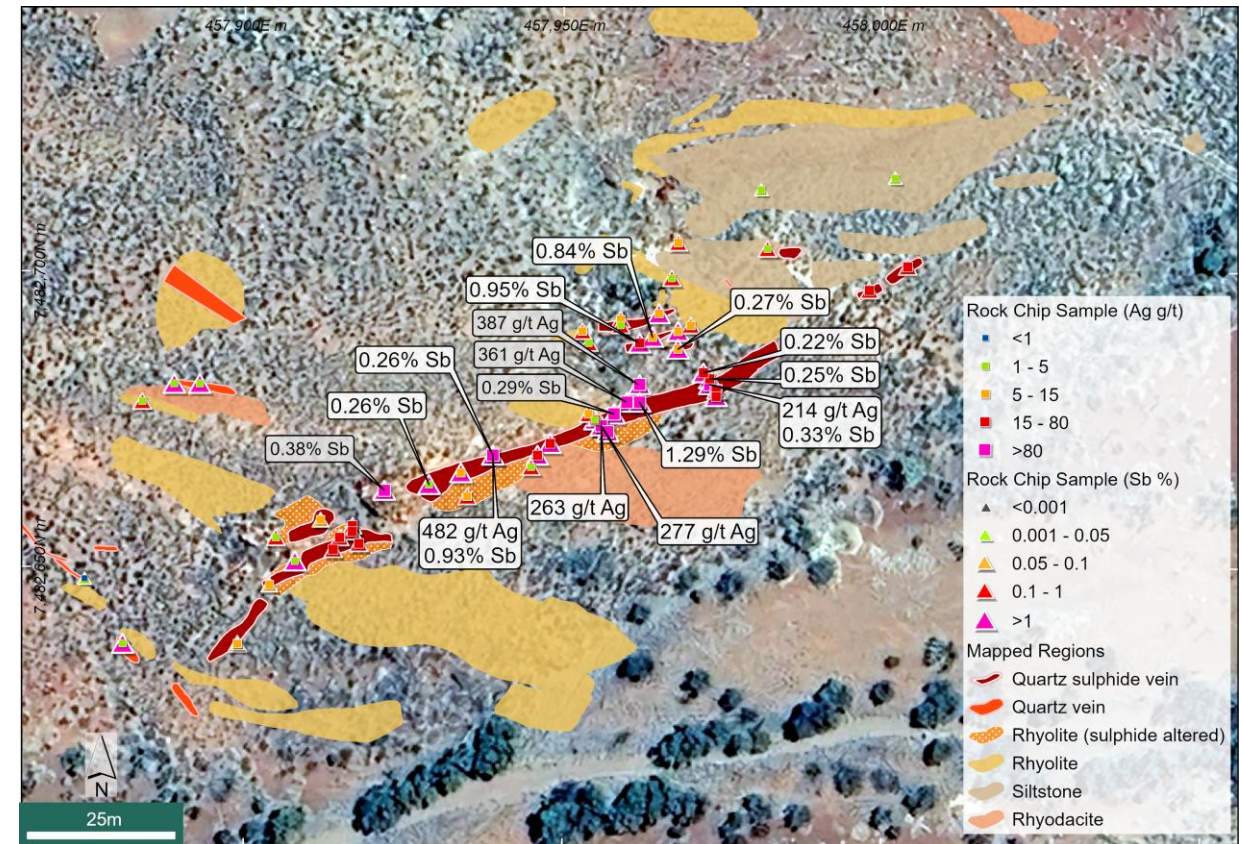
Geological mapping and significant Sb and Ag rock chip results at the SE Wyloo prospect 9,10
