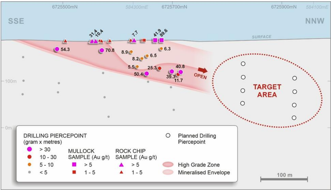
Clone long section with surface rock chip results, and drilling pierce points with planned follow-up RC drilling pierce points (white dots) 3
