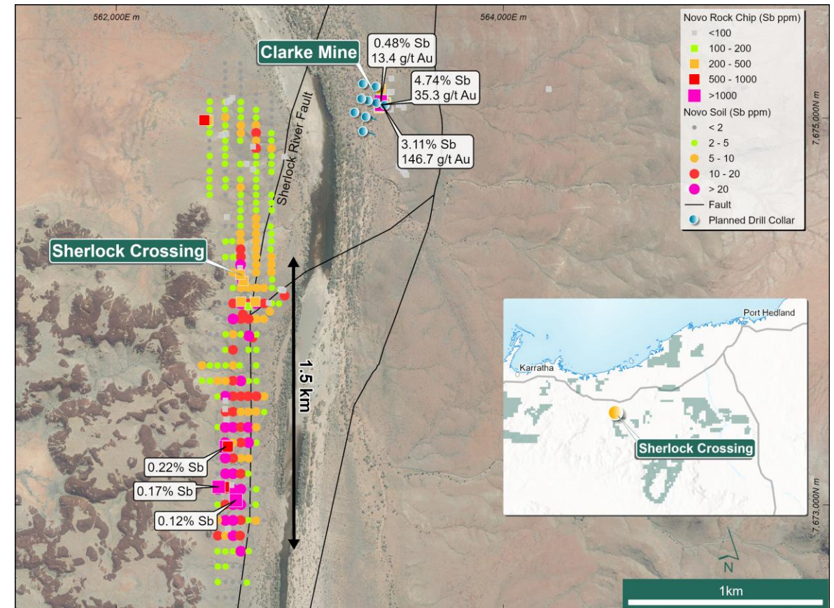
Sherlock Crossing, showing extended soil anomaly > 15 ppm Sb to the SW of the proposed first pass drilling area at the Clarke Mine 8
