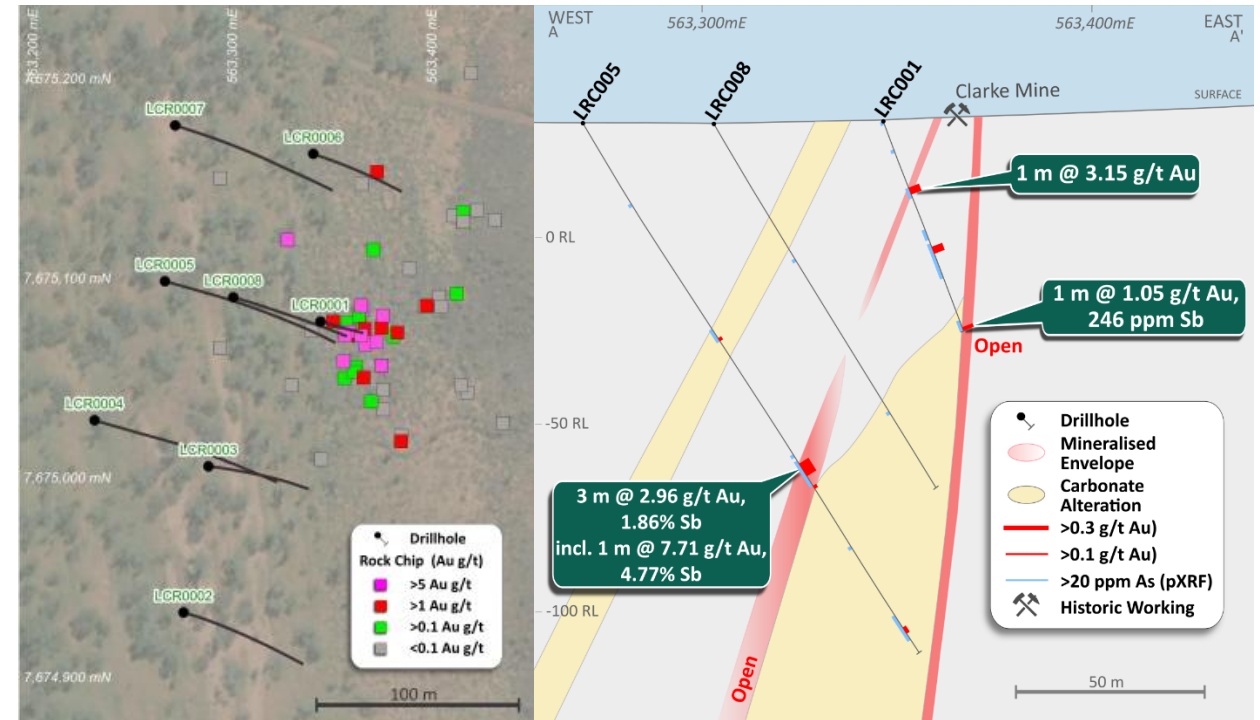
Sherlock Crossing RC drill plan with rock chip results and cross section showing key Au-Sb intercepts and As geochemistry Carbonate alteration is strengthening and mineralisation is open at depth 6 .
