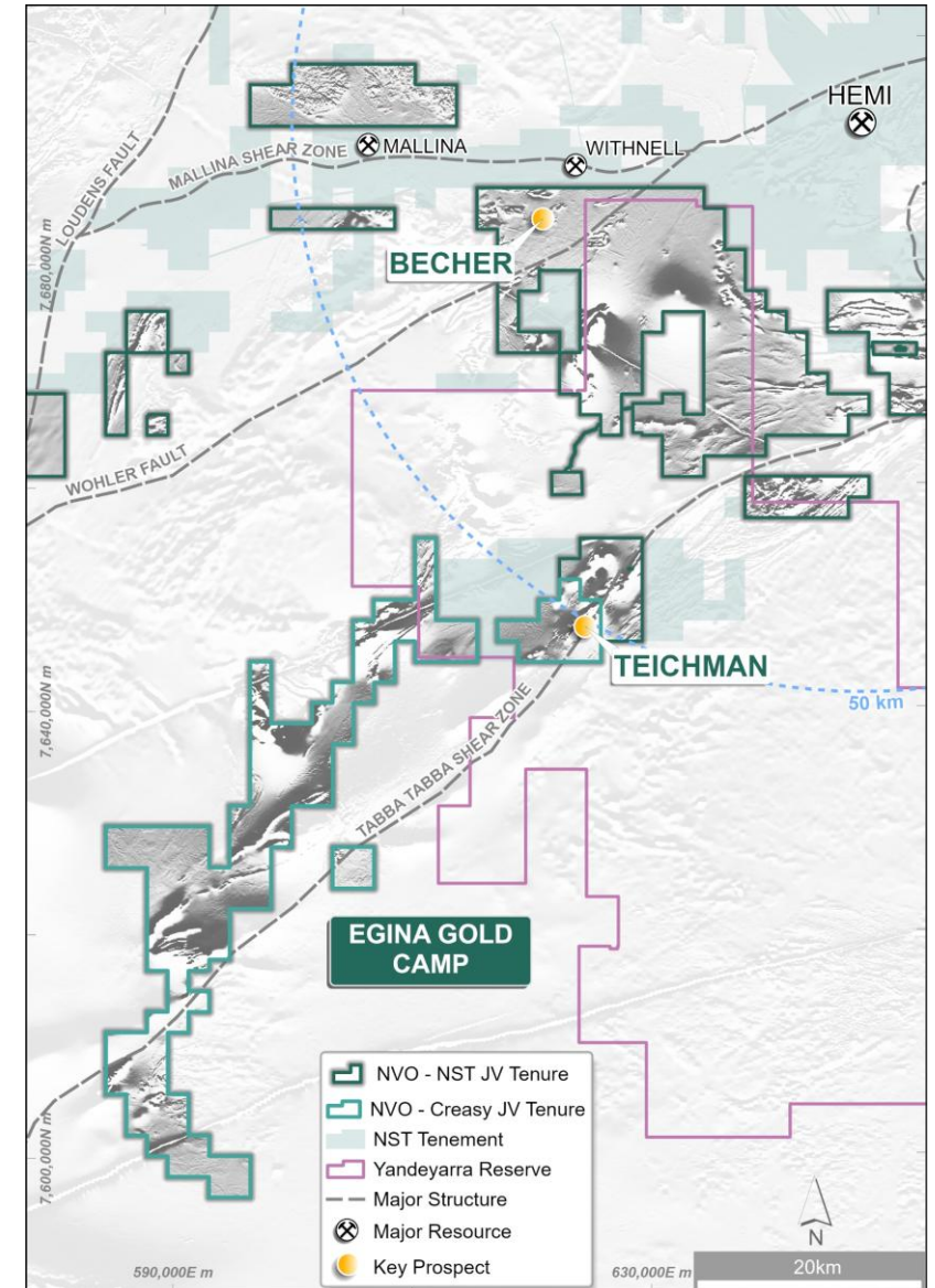
Location of Egina Gold Camp tenements and major prospects
