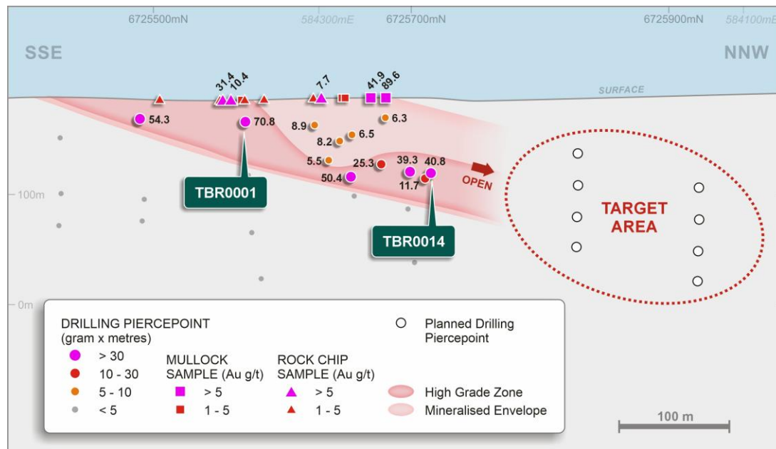
Clone long section with surface rock chip results, and drilling pierce points with planned follow-up RC drilling pierce points (white dots) 12
