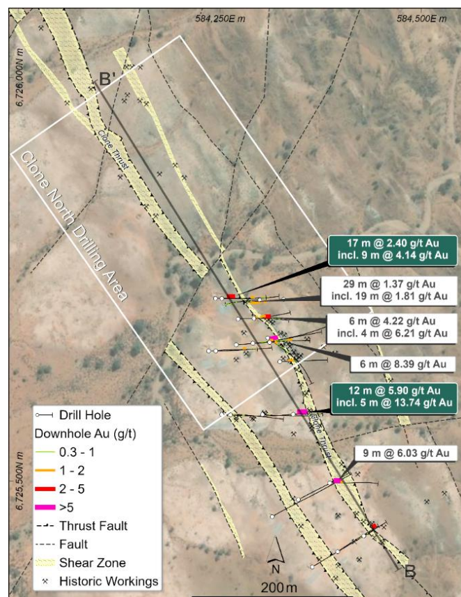
Figure 2: Targeted mineralised structures and alteration zones at the Clone prospect, showing previous drilling with significant intercepts by Novo 1 (larger collars, green callouts) and previous drilling with significant intercepts by Manhattan 1 (smaller collars, white callouts). Area of upcoming drilling at Clone is also demarcated.
