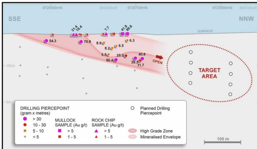
Figure 3: Clone interpreted long section (B {SSE} – B' {NNW}) - see Figure 1 for location) highlighting grade and width continuity, shallow north plunge to the high-grade defined shoot, and the down plunge current target to the mineralisation that is open to the north. Pierce points represent drill intersections expressed in gram x metre values from both the Manhattan 2023 RC 1 and Novo 2025 RC 1 drill programs. Planned new RC drill collars in white are schematic albeit broadly in line spatially with planned step out drill lines at 100 m and 200 m respectively to the north of existing drilling.
