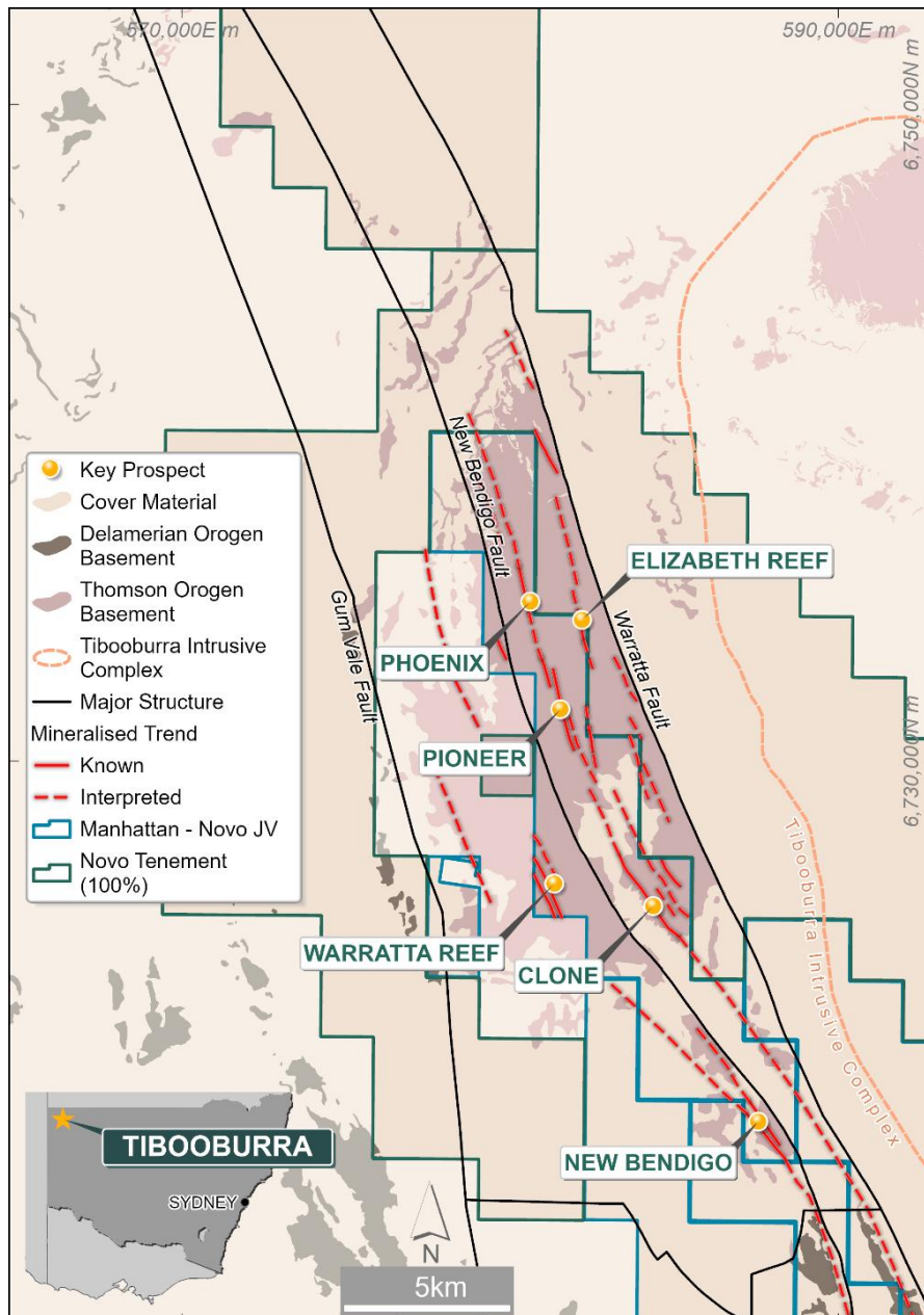
Figure 4: The Tibooburra Gold Project showing basement geology (darker colours) versus younger cover sequences (lighter colours) and key structural architecture. Solid red lines represent known mineralised trends; dashed red lines are interpreted mineralised trends. Only key prospects are depicted.
